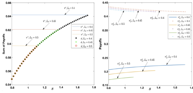
Fig. 5. Sum of equilibrium-type solution payoffs \pi^* , sum of disagreement payoffs d (left), individual payoffs (right) versus s .
