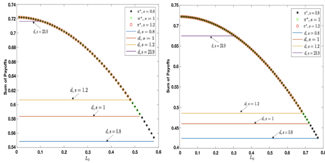
Fig. 2. Sum of equilibrium-type solution payoffs of SPs, \pi^* , when \Delta = -0.5 (left) and when \Delta = 0.5 (right) versus L_0 , sum of disagreement payoffs of SPs is d .
