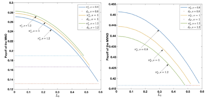
Fig. 3. Equilibrium-type solution and disagreement payoffs of SP_L (left), SP_F (right) when \Delta = -0.5 versus L_0 .
