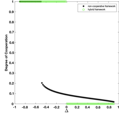
Fig. 1. The degree of cooperation versus \Delta .
