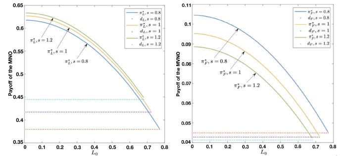
Fig. 4. Equilibrium-type solution and disagreement payoffs of SP_L (left), SP_F (right) when \Delta = 0.5 versus L_0 .
