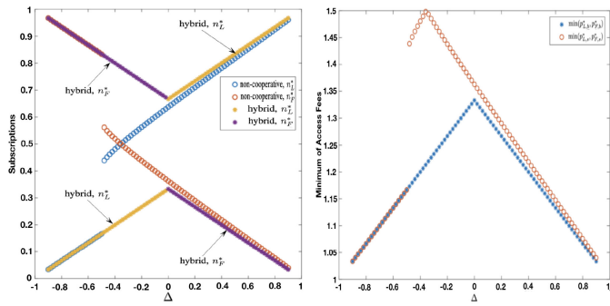
Fig. 6. The subscriptions (left), the access fees (right) versus \Delta .
