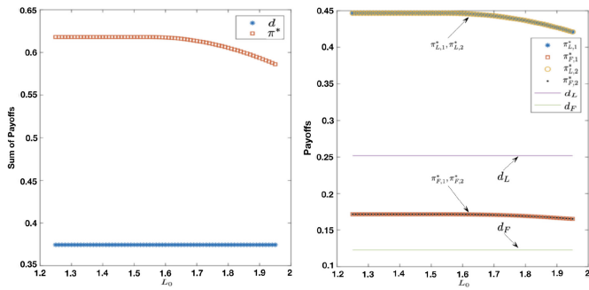
Fig. 9. Sum of equilibrium-type solution payoff, \pi^* , disagreement payoff, d (left), payoffs of individual SPs (right) versus L_0 .
